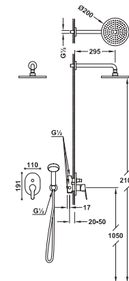
Concealed shower set with water shut off and flow control. · Fixed shower head Ø 200 mm, with ball joint. · Elbow wall. · Antilime hand shower. · Hand shower hose.
